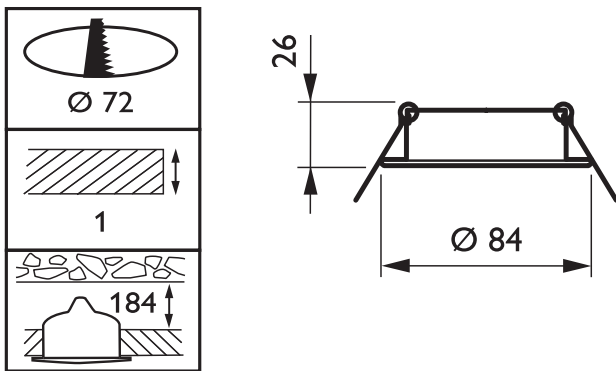
QBS032 1x MAX50W-GU5.3 12V SI
