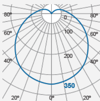
Integrated LED Luminaire F29100SM-3000K
