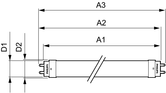
TLED 220-240V 10-18W 3000K G13 EcoFit
