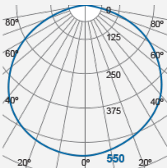
Integrated LED Luminaire F50100SMv1
