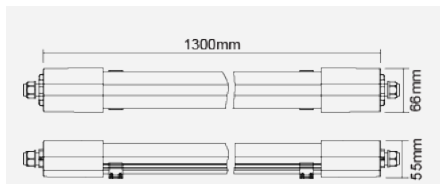
Integrated LED Luminaire F50100SMv1
