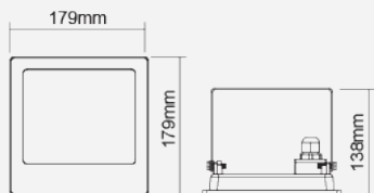
Integrated LED Luminaire FFL70200v0
