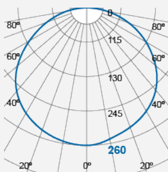
Integrated LED Luminaire FIB71500v0-3000K
