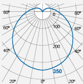
Integrated LED Luminaire FIB71600v0-3000K
