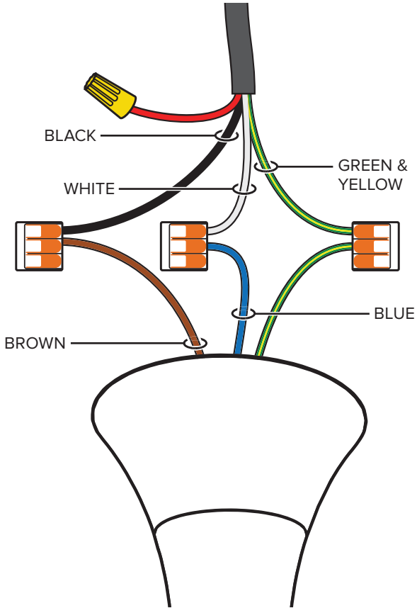
Wiring Diagram
